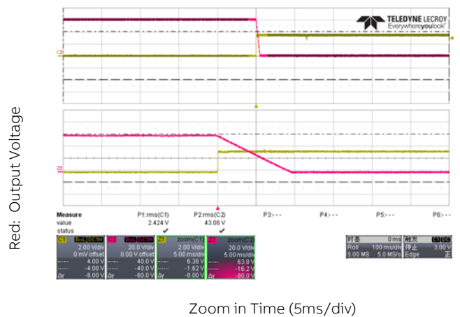
Figure 18. PG# alarmed 10ms prior to V_o < 40V , V_{IN} = 230V_{AC} , Output at Full load
